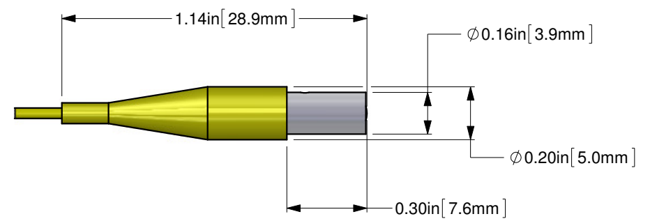
DETAIL A
