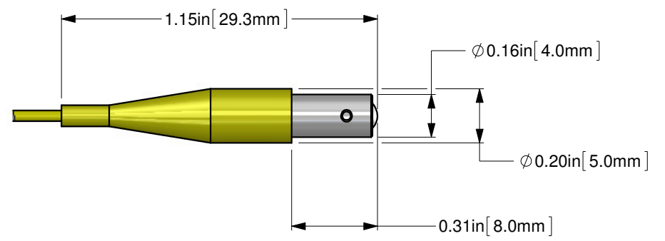
DETAIL A
