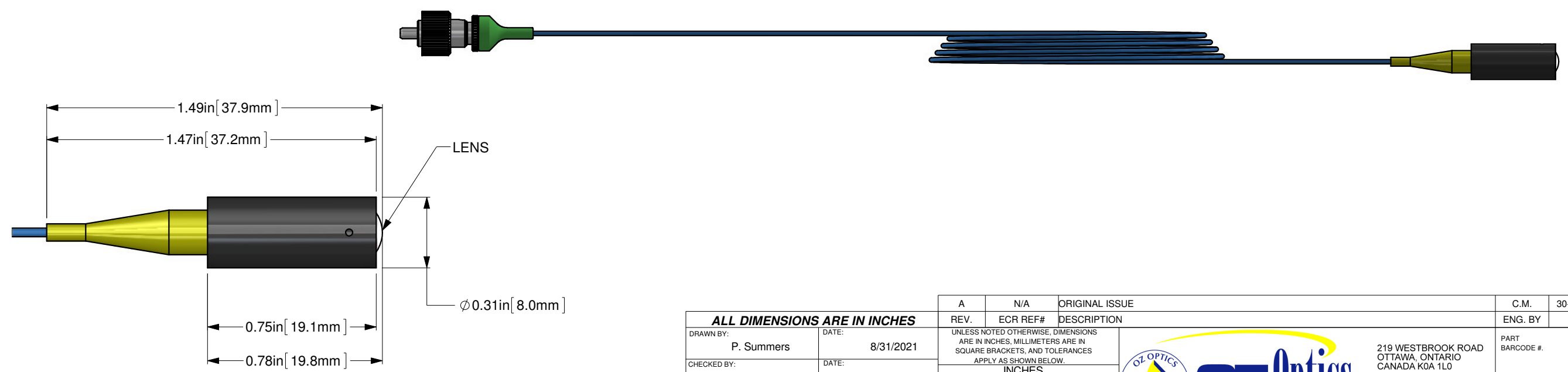
DETAIL A
