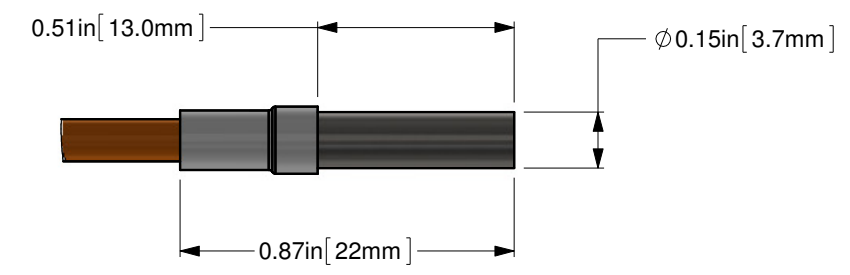
DETAIL A
